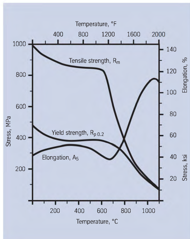
Fig. 1 – Typical short-time mechanical properties at elevated temperatures of cold rolled Nicrofer 6020 hMo annealed at 1000 °C (1830 °F).
