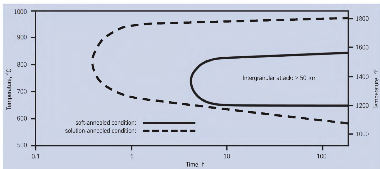
Fig. 2 – Time-Temperature-Sensitization (TTS) diagram for Nicrofer 6020 hMo (0.02 % carbon) according to ASTM G-28 A, (120 h).
